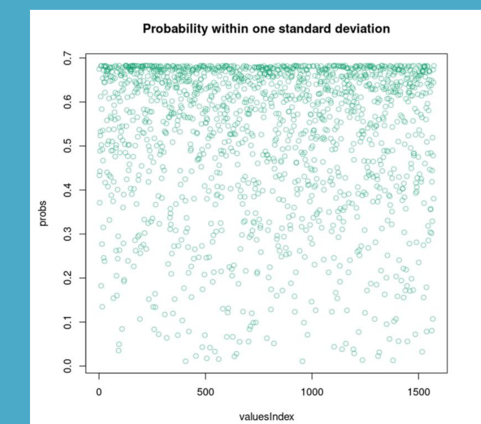
Data points' probabilities that indicate if they're outliers.
